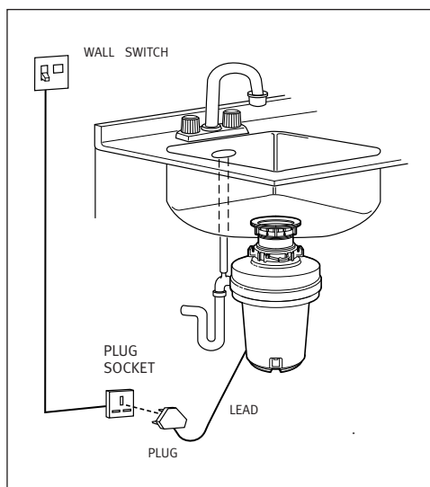
Wall Switch Installation Illustration
